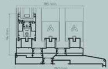
250 mm Subcill
